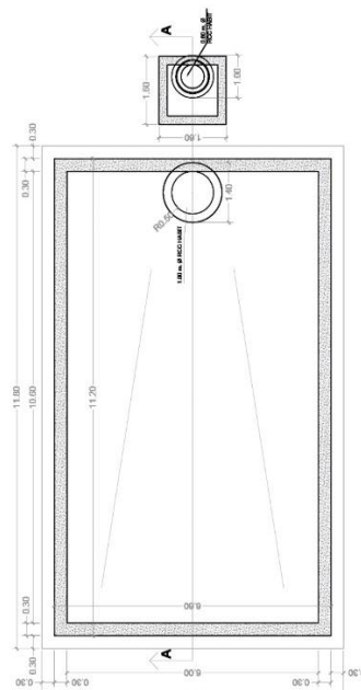
RAINWATER HARVESTING TANK PLAN ( 1:70 )
