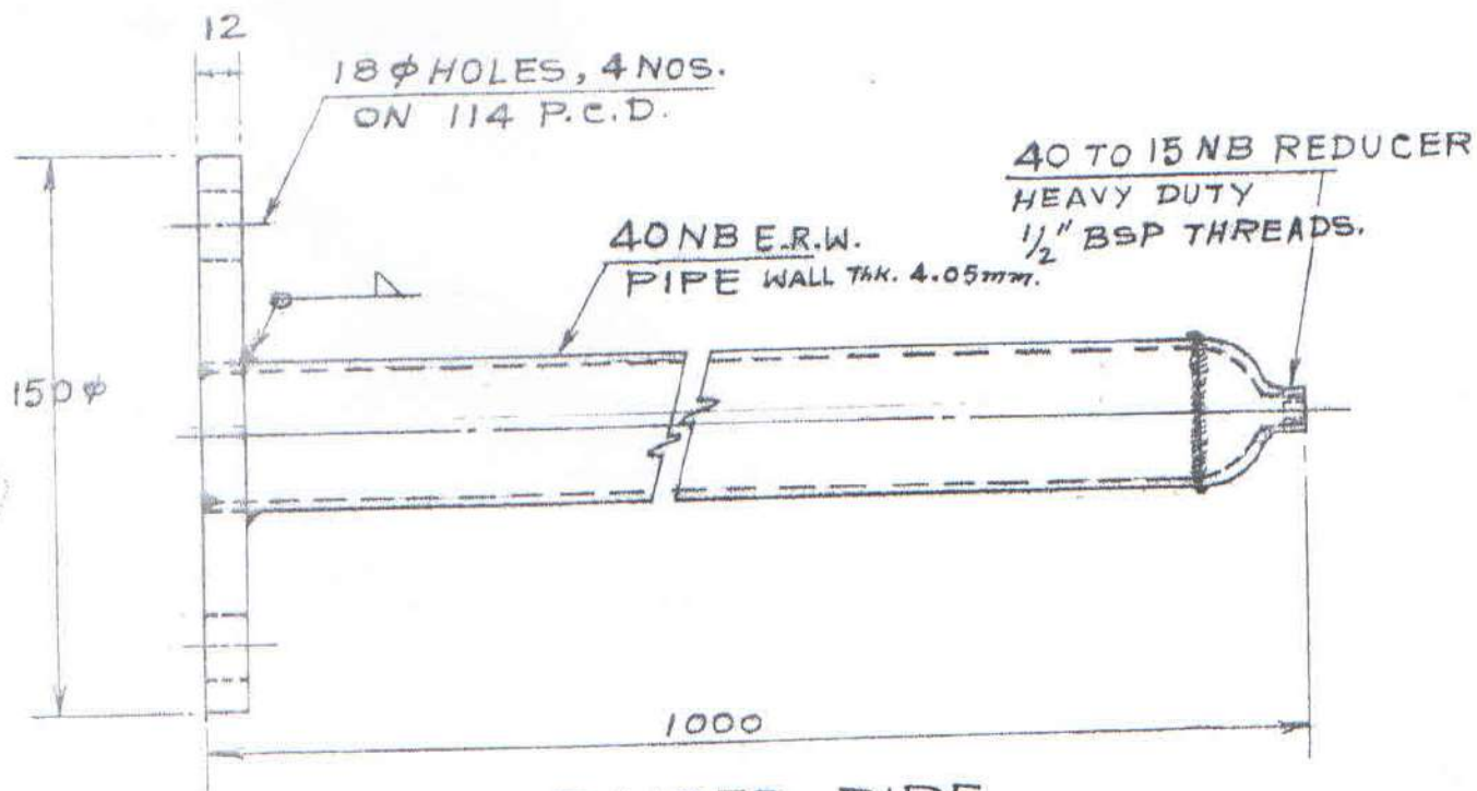
RAISER PIPE
