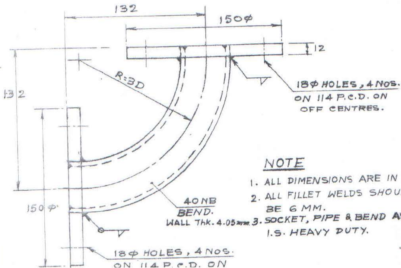
RAISER PIPE
