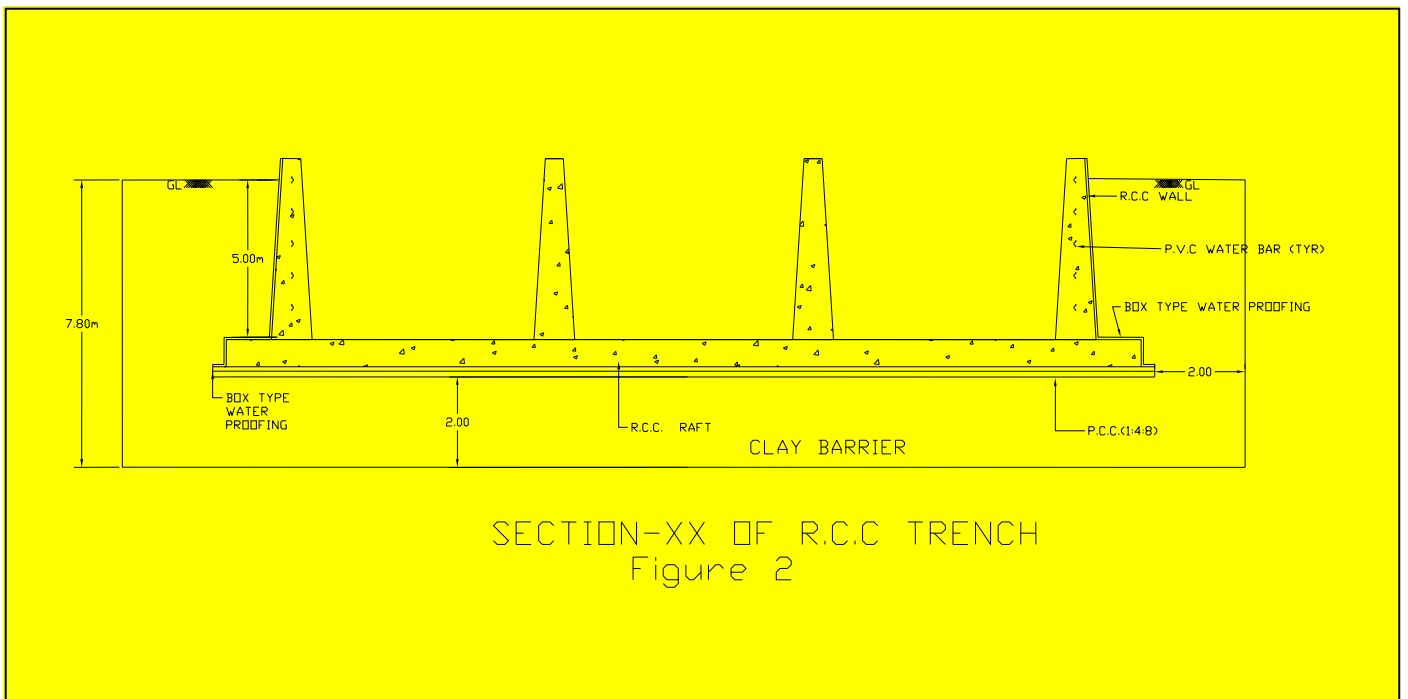
Typical section of trench
