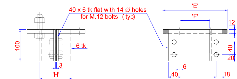
VIEW Y-Y
