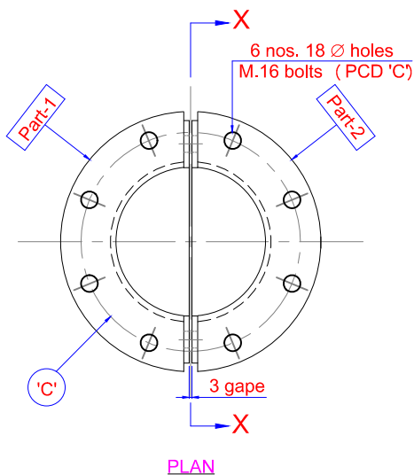
Figure - 1 (For 140 Ø & 160 Ø PIPES)
