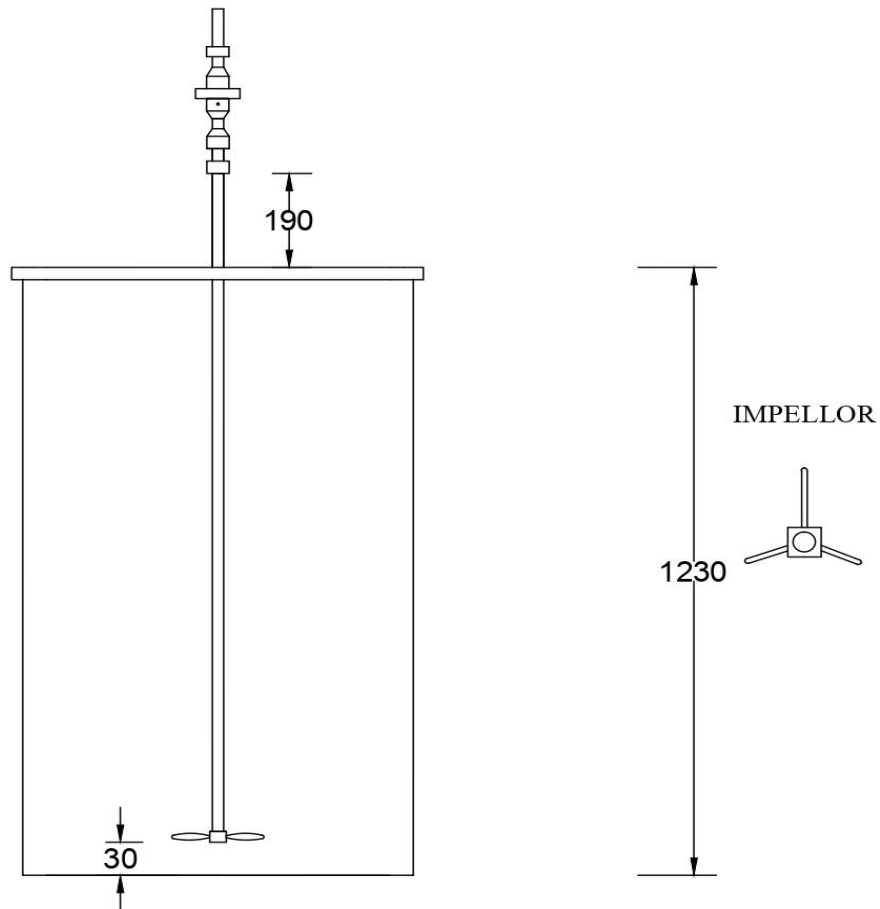
SECTIONAL VIEW
