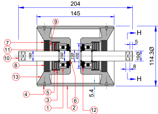
SECTIONAL VIEW FOR INTERNAL DETAILS CARRYING IDLER
