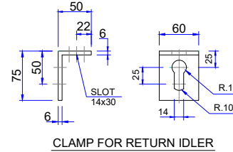
CLAMP FOR RETURN IDLER
