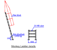
Monkey Ladder details
