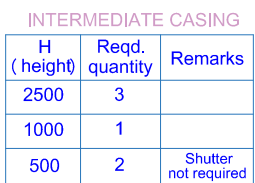
DETAILS OF INTERMEDIATE CASING
