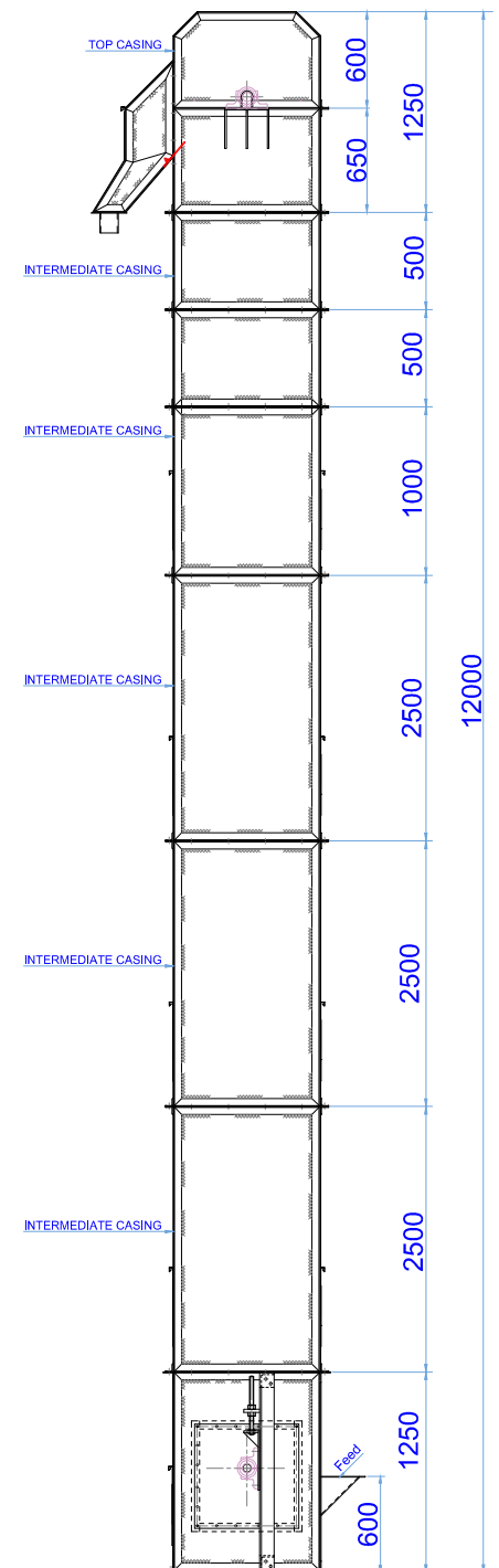
ASSEMBLED VIEW OF ELEVATOR
