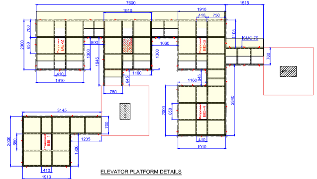
ELEVATOR PLATFORM DETAILS
