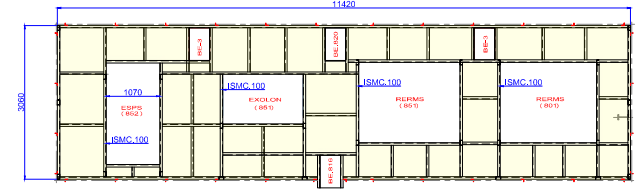
PLAN Working platform ( Height 5.350 mtr )
