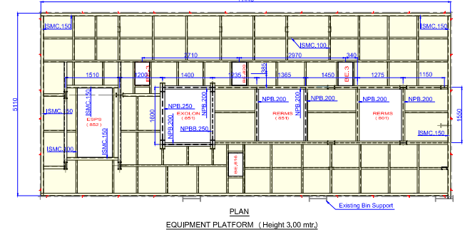
PLAN EQUIPMENT PLATFORM ( Height 3.00 mtr )
