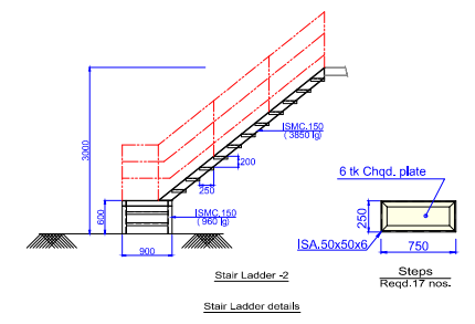
Stair Ladder details
