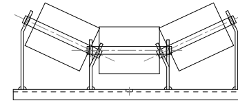
FRAME FOR CARRYING IDLER
