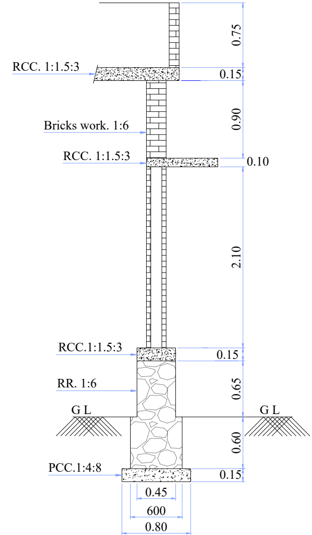
FOUNDATION DETAILS
