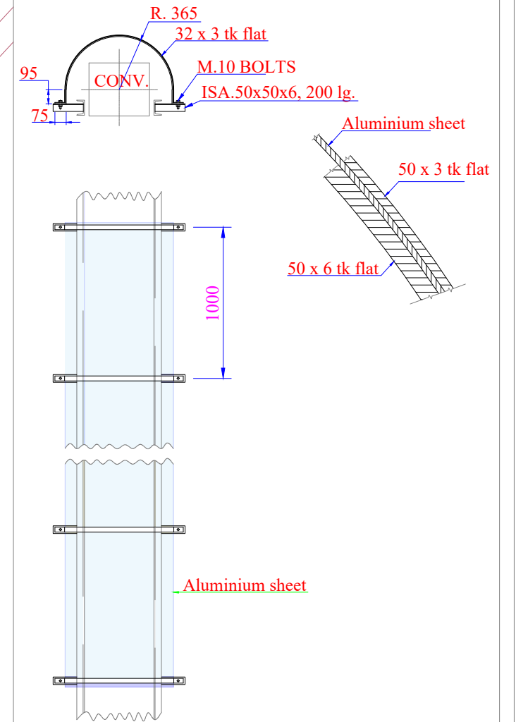
CONVEYOR COVERING DETAILS
