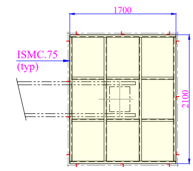
PLATFORM FOR CONVEYOR HEAD END (Required 3 sets for BC.2, 3 & BC 304)
