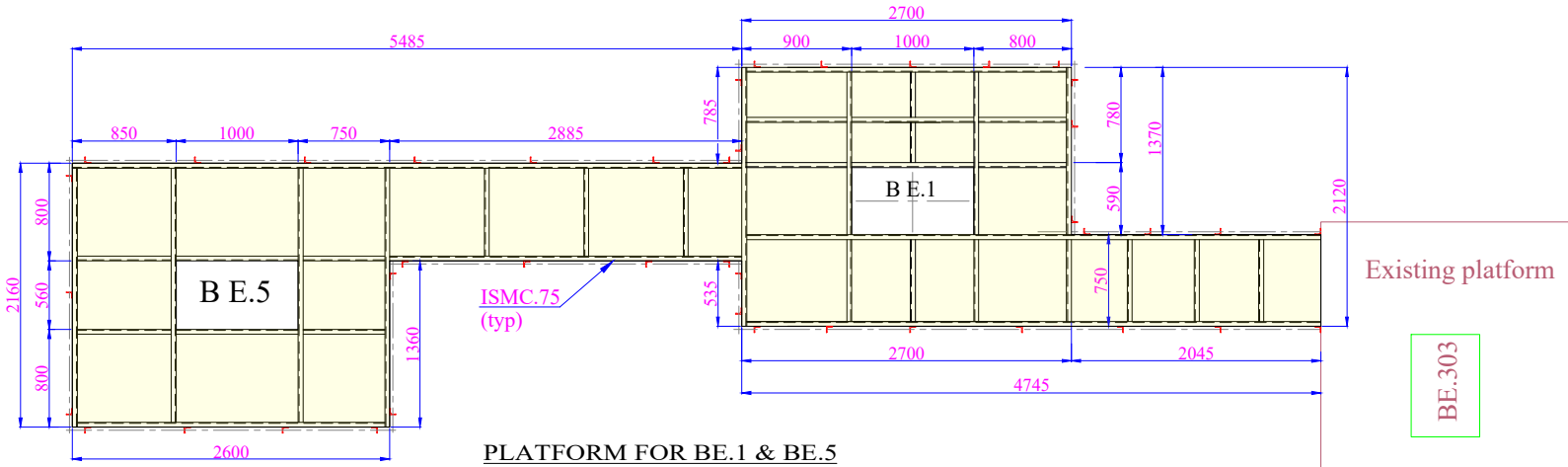
PLATFORM FOR BE.1 & BE.5
