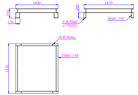
RERMS MOUNTING STAND (REQD. 1 No.)
