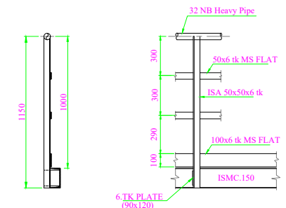
TYPICAL HAND RAILS DETAILS
