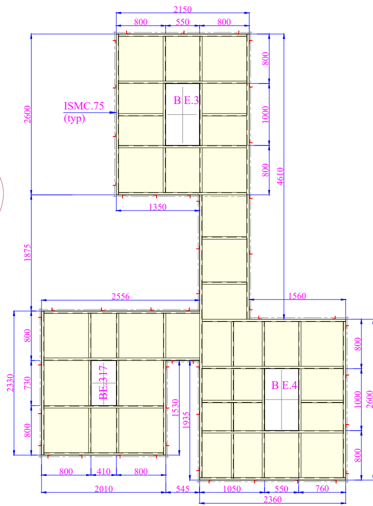
PLATFORM FOR BE.2, 3 & BE.317
