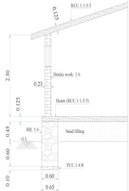
FOUNDATION DETAILS
