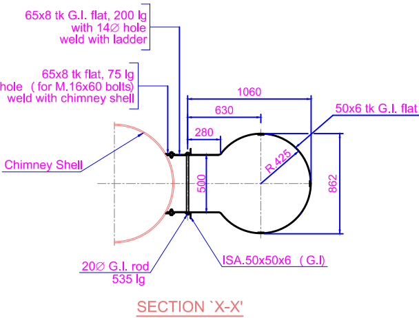
SECTION 'X-X'
