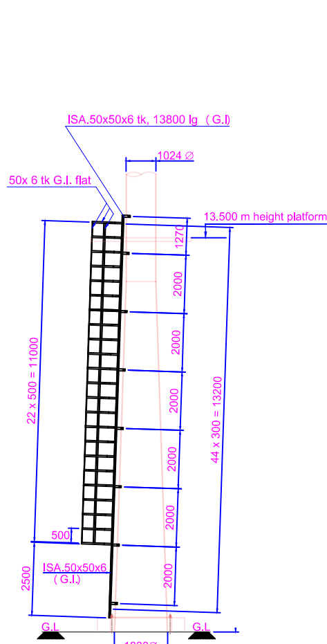
DETAIL OF PART MKD. "E" (Monkey Ladder with cage)
