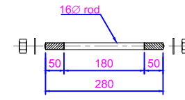
DETAIL - C
