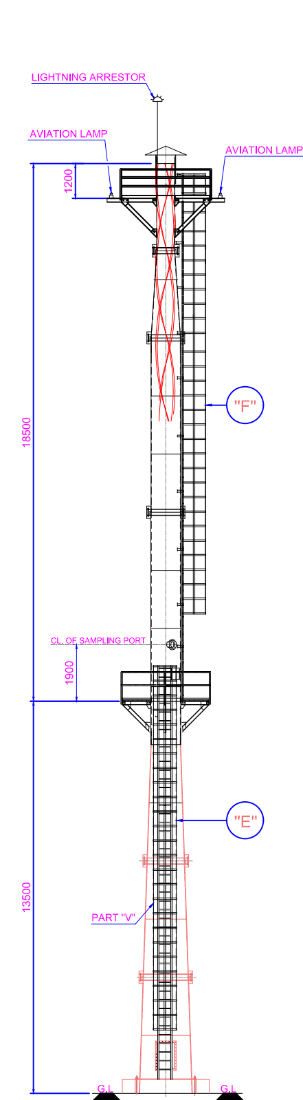
CHIMNEY GENERAL ARRANGEMENT
