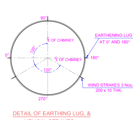
DETAIL OF EARTHING LUG, & HELICAL STRAKES
