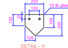
DETAIL - H
