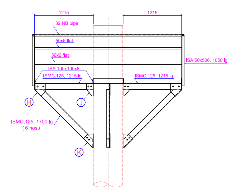
PLATFORM SUPPORTING DETAILS
