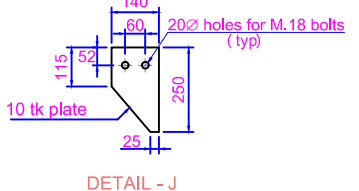
DETAIL - J
