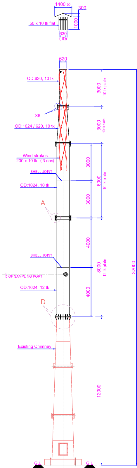
CHIMNEY DETAILS
