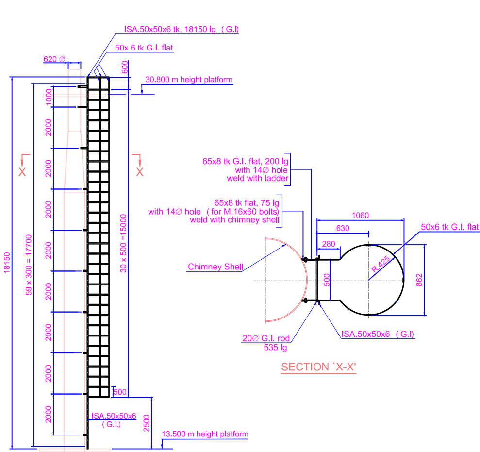
DETAIL OF PART MKD. "F" (Monkey Ladder with cage)
