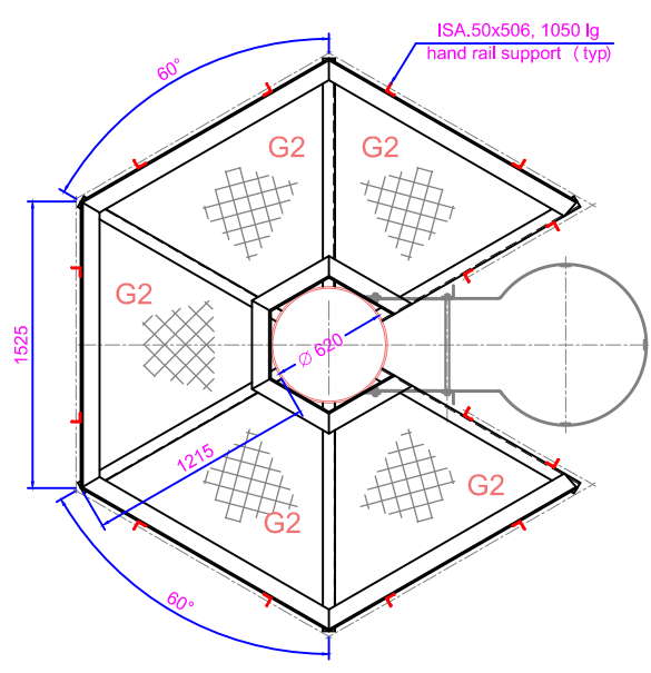
PLATFORM AT 30.800 mtrs. HEIGHT
