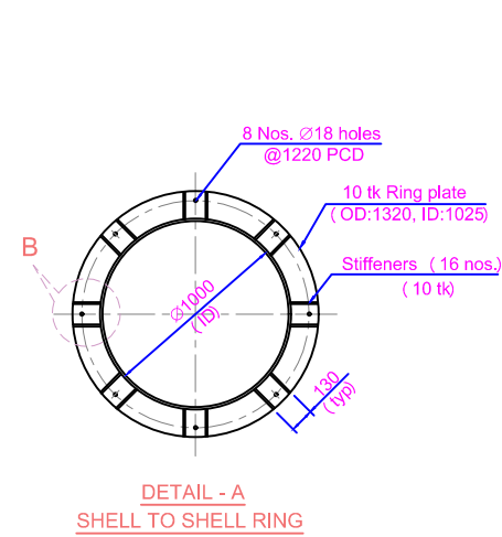
DETAIL - A SHELL TO SHELL RING
