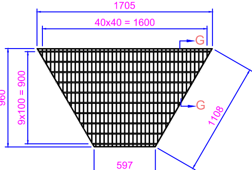
GRATING DETAIL G1 : 5 Nos.
