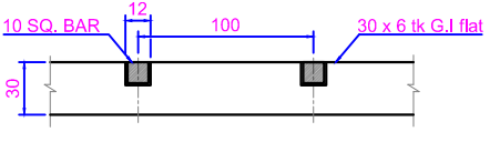
SECTION 'G-G'
