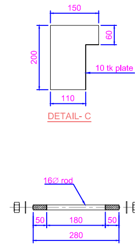
DETAIL - C
