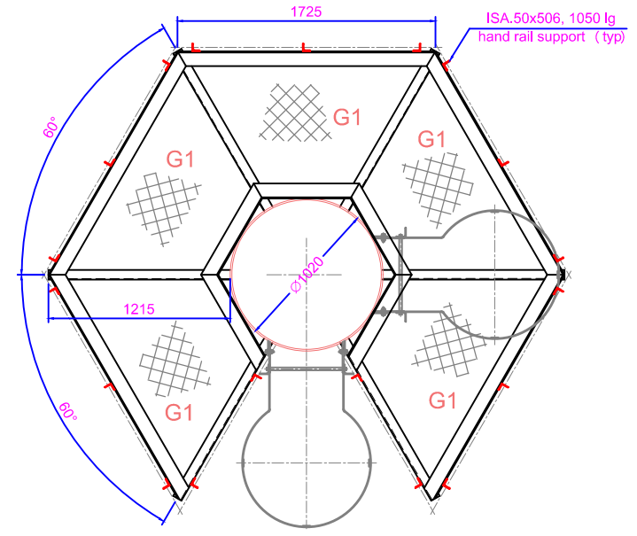
PLATFORM AT 13.500 mtrs. HEIGHT
